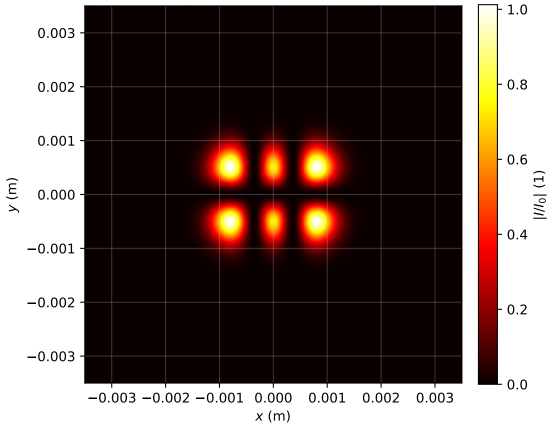
Intensity profile I(x, y, z = 0.398)/I_0 , P_{in}=0.5P_{cr} , artificial time
